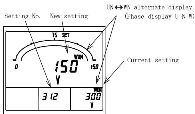
Phase-voltage full scale (1 \phi 3W)
