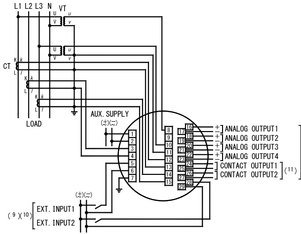
(1) Voltage, Current input (2VT, 3CT)
