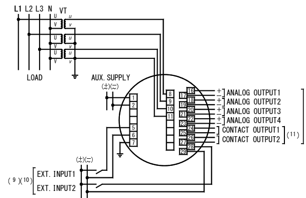
(5) Voltage input (3VT)
