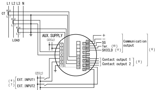
(3) Current input
