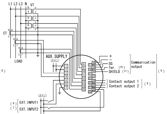
(2) Voltage, Current input (3VT, 3CT)
