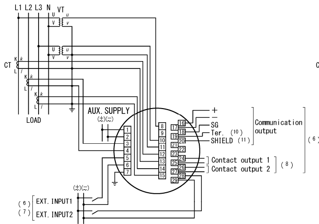
(1) Voltage, Current input (2VT, 3CT)
