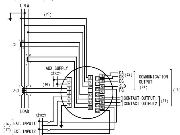
(2) 1P3W (N-phase earth)
