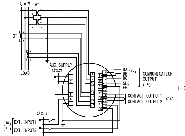
(5) Current input 3P3W (2CT)
