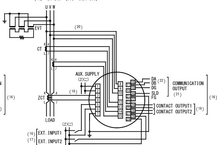
(4) 3P3W (No earth)
