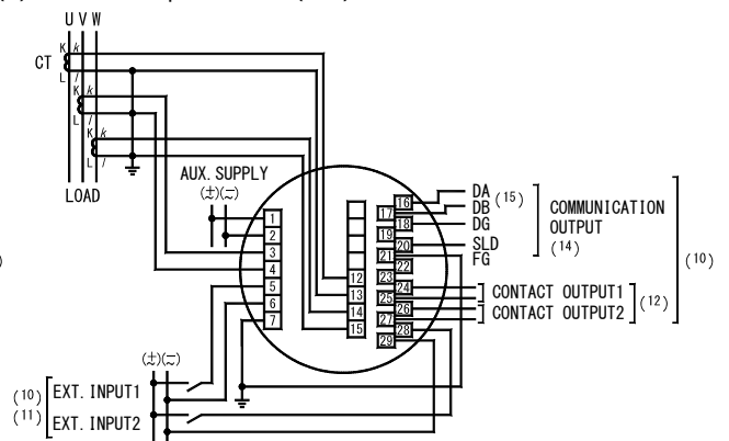
(6) Current input 3P3W (3CT)
