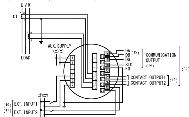
(5) Current input 3P3W (2CT)
