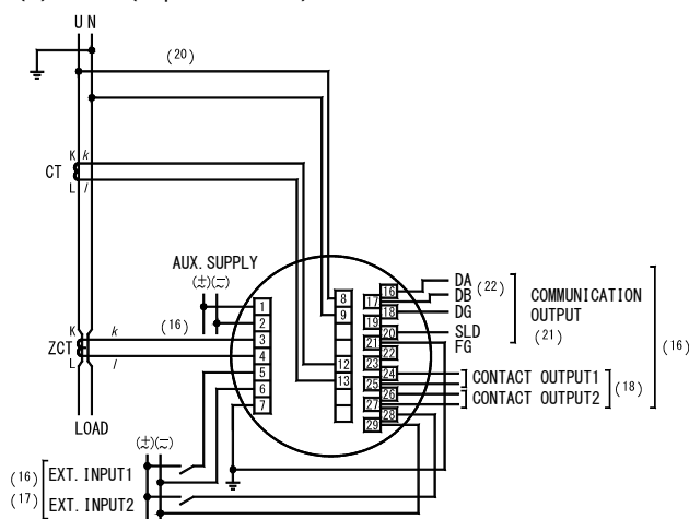
(1) 1P2W (N-phase earth)
