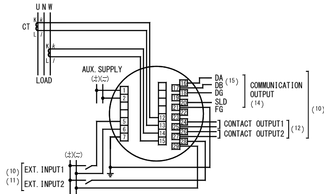
(7) Current input 1P3W
