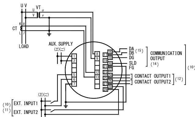
(3) 3P3W (2VT, 2CT)
