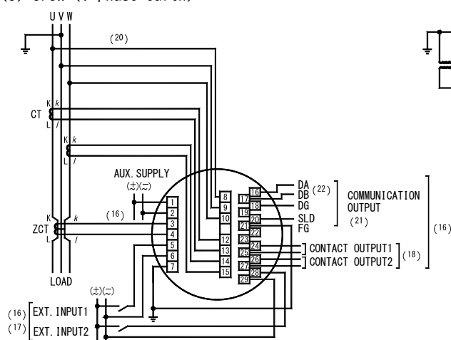
(3) 3P3W (V-phase earth)
