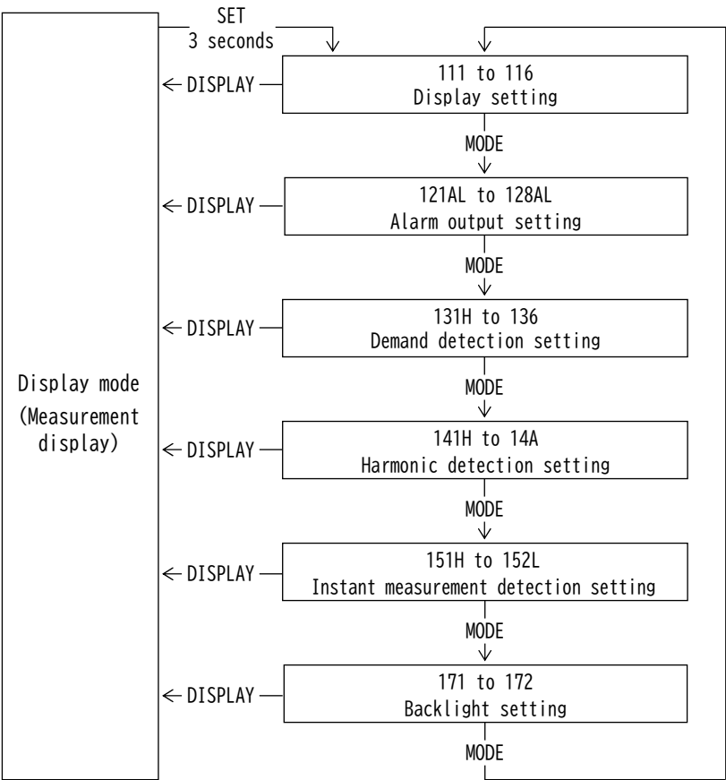
Setting mode 1
