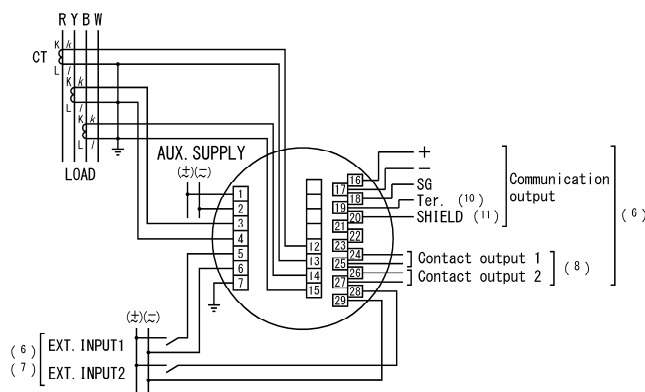
(3) Current input
