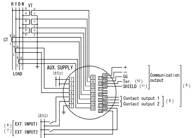
(2) Voltage, Current input (3VT, 3CT)
