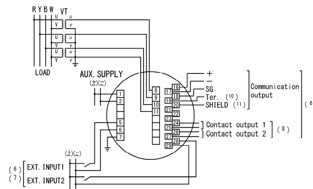
(5) Voltage input (3VT)
