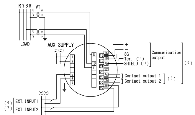
(4) Voltage input (2VT)
