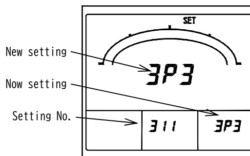
Setting mode 3 (No.311 Input circuit phase line change)
