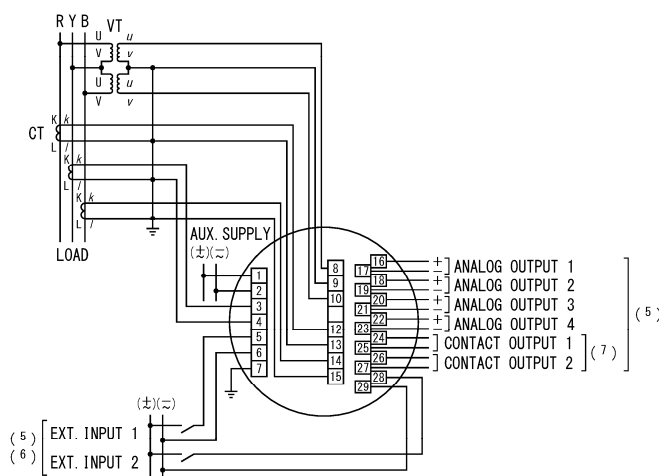
(1) 3P3W (2VT, 3CT)
