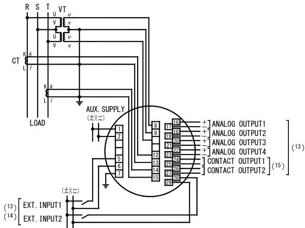
(3) 3 φ 3W (2VT, 2CT)
