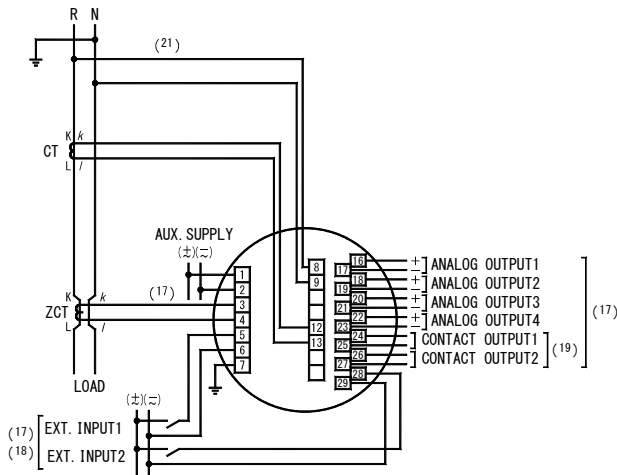
(1) 1 φ 2W (N-phase grounding)
