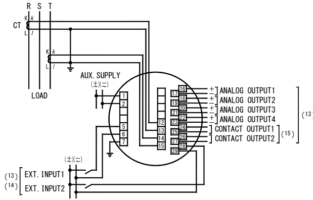
(5) Current input 3φ3W (2CT)
