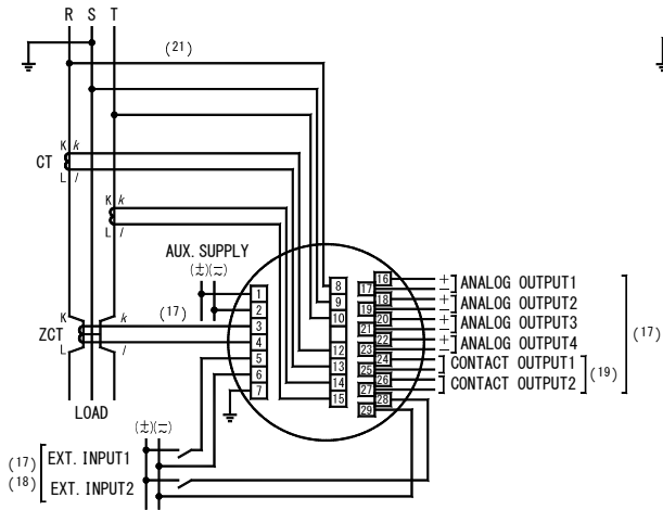
(3) 3 φ 3W (S-phase grounding)
