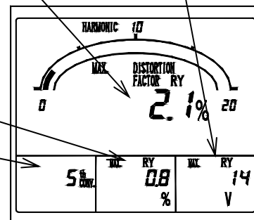
Voltage harmonic measurement maximum display.
