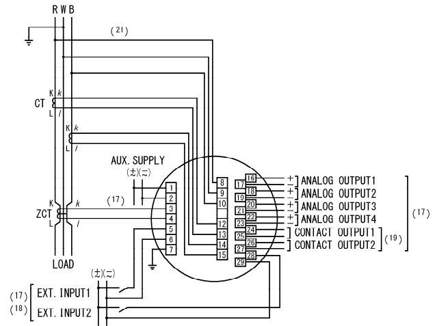
(2) 1P3W (W-phase grounding)
