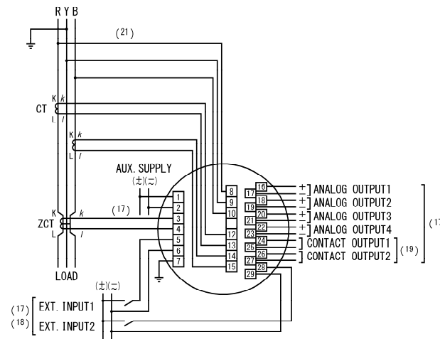
(3) 3P3W (Y-phase grounding)
