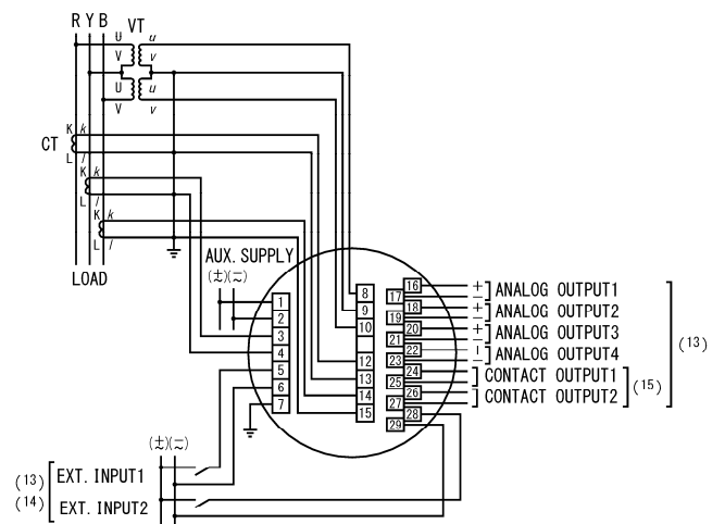
(4) 3P3W (2VT, 3CT)
