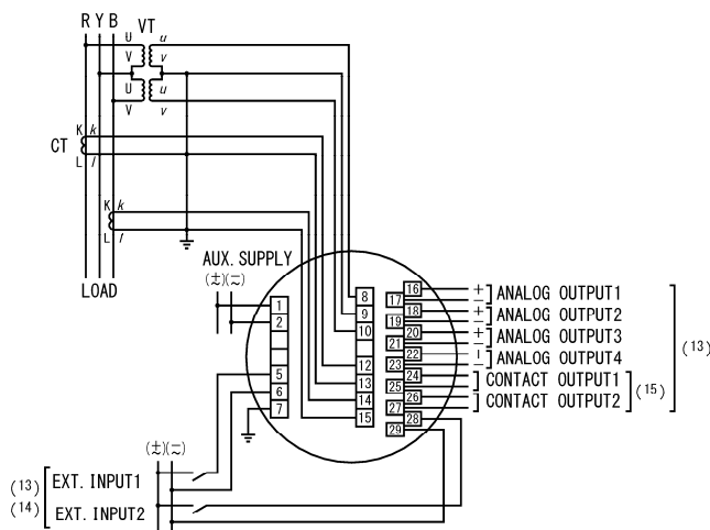
(3) 3P3W (2VT, 2CT)
