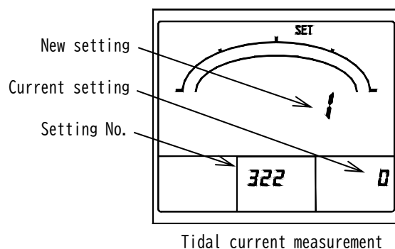
Dead band of measurement
