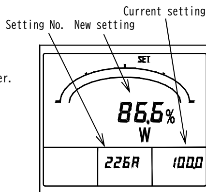
Active power output intrinsic sensitivity
