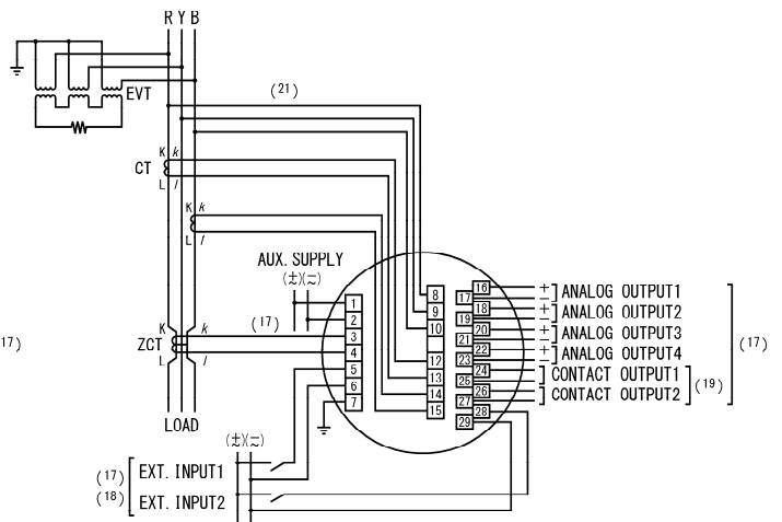
(4) 3P3W (No grounding)
