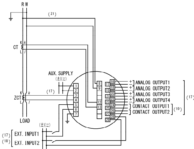
(1) 1P2W (W-phase grounding)
