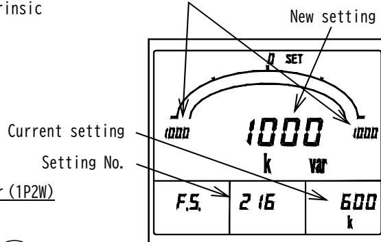
Reactive power display intrinsic sensitivity
