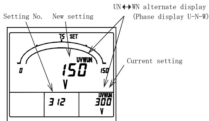
Phase-voltage full scale (1 \phi 3W)
