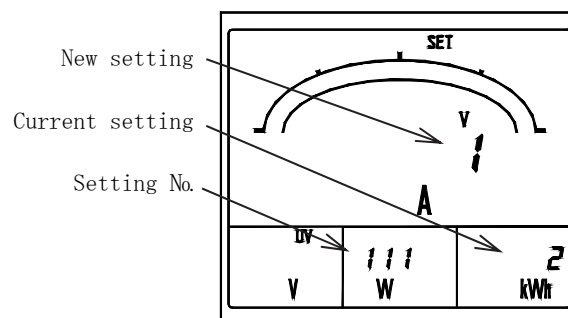
Combination display
