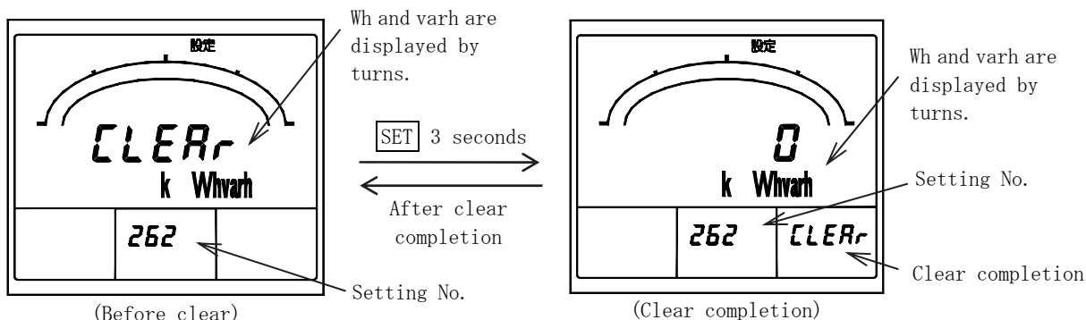
Watt-hour reset
