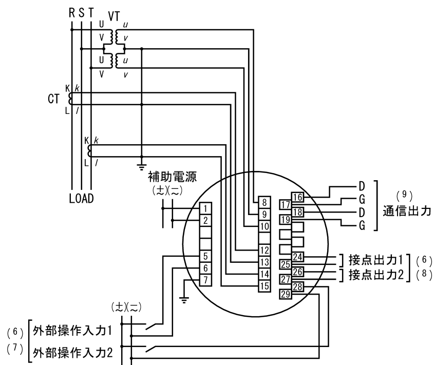
(3) 3 \phi 3W (2VT2CT)
