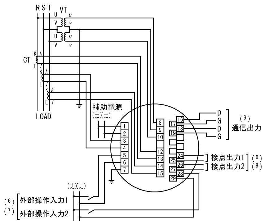
(4) 3 \phi 3W (2VT3CT)
