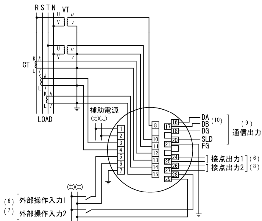
(5) 3 \phi 4W (2VT3CT)
