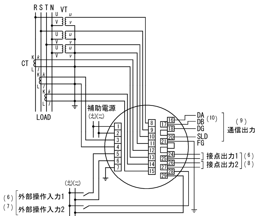
(6) 3 \phi 4W (3VT3CT)
