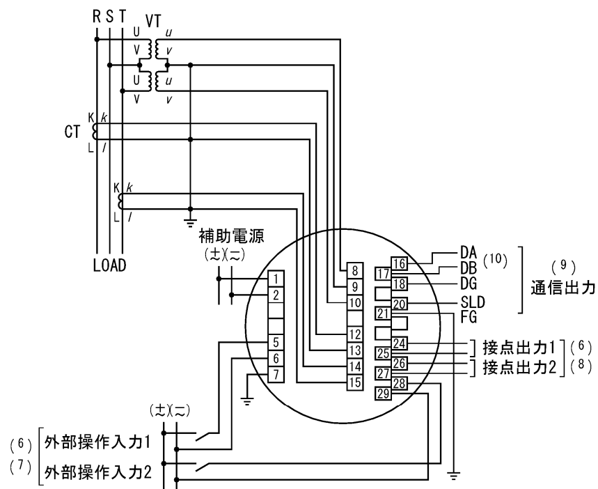
(3) 3 \phi 3W (2VT2CT)
