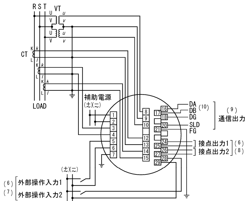
(4) 3 \phi 3W (2VT3CT)
