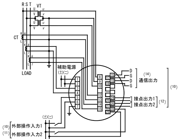
(4) 3φ3W (2VT, 3CT)
