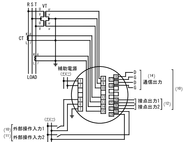
(3) 3φ3W (2VT, 2CT)
