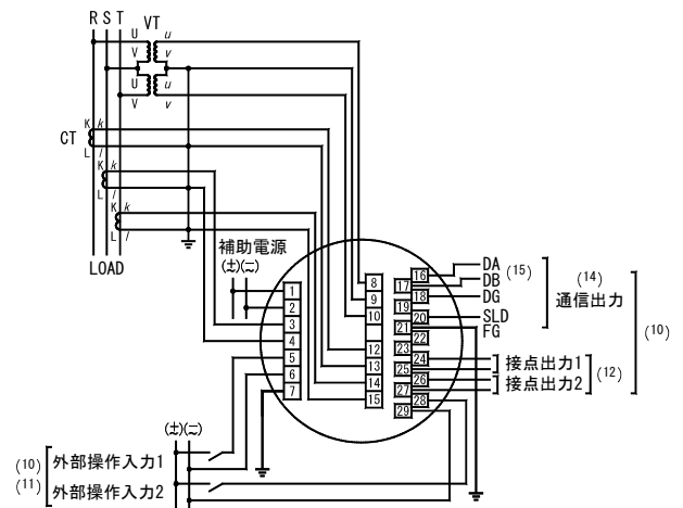
(4) 3φ3W (2VT, 3CT)
