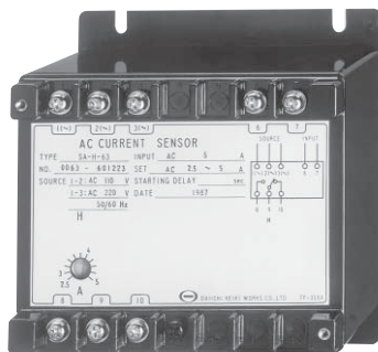
SA-H-63 (120×110×112mm/0.7kg)
