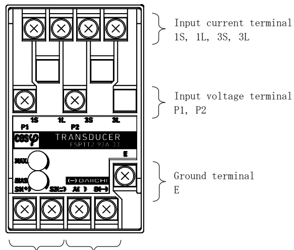
Auxiliary supply terminal Output terminal S1(±), S2(±) A(+), B(-)
