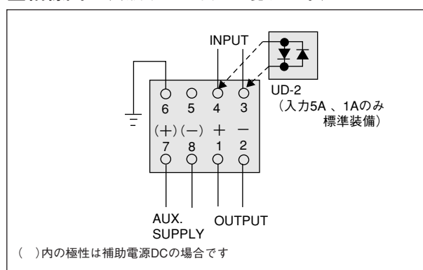
AETP2-3F2 (108(UD-2付)×50×121mm/450g)
